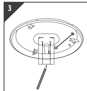
3 Ensure product is located in the correct location and mark the fixing surface
